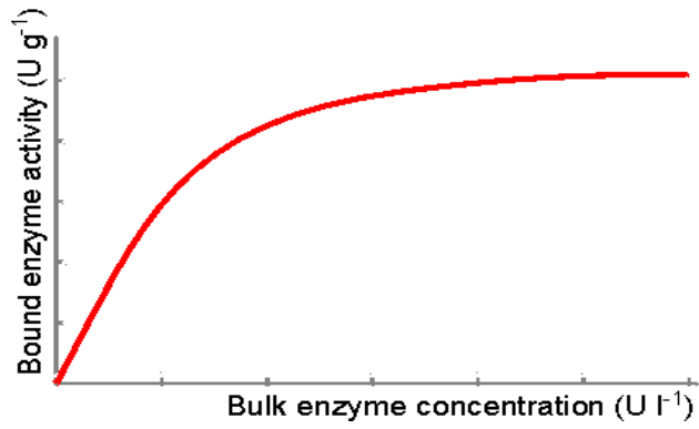
ENZYME CONCENTRATION
